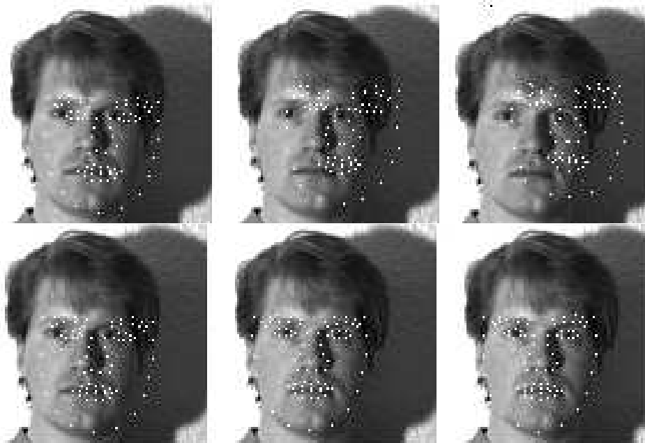
Fig. 8. Sensitivities of AAM (upper) and TC-ASM (lower) to illumination condition not seen in the training data. From left to right are the results obtained at the 0-th, 2-th, and 10-th iterations. (Result in different level of image pyramid is scaled back to the original scale)
